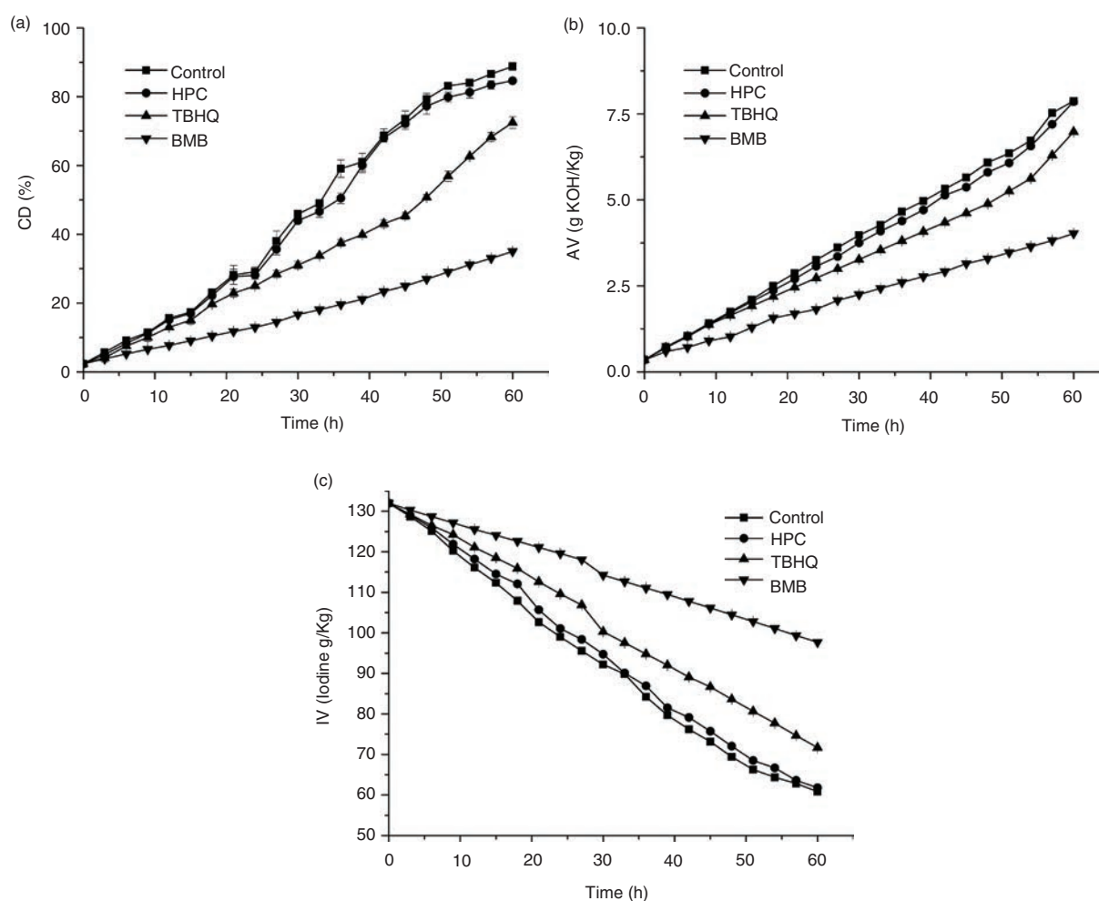
FIGURE 4. Changes in percentage conjugated diene (CD), acid (AV) and iodine (IV) values in oil samples during deep frying at 180 °C. Values are expressed as Mean \pm SD (n=2). Statistical significance at p \leq 0.05 .
