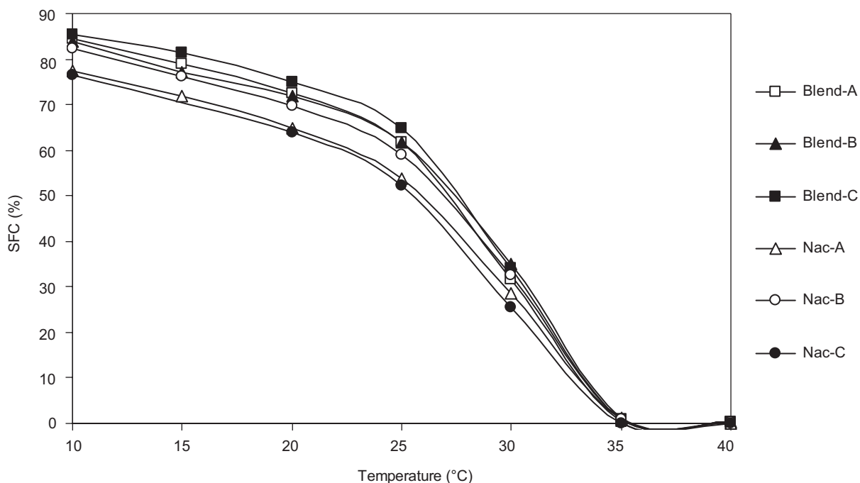
Figure. 1 Solid fat content profiles of the cocoa butter samples.
