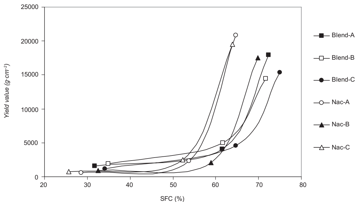
Figure 2 Relation between yield value and solid fat content of the cocoa butter samples at 20, 25 and 30 °C.
