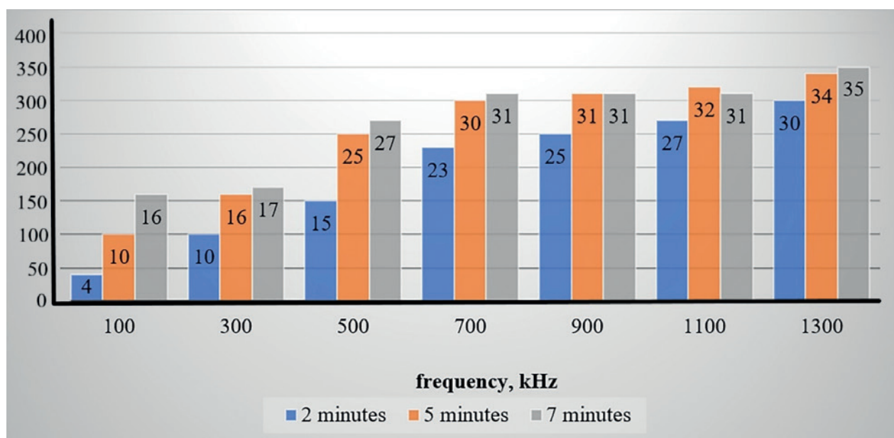
FIGURE 2. How emulsion stability is affected by alterations in processing frequency and duration
